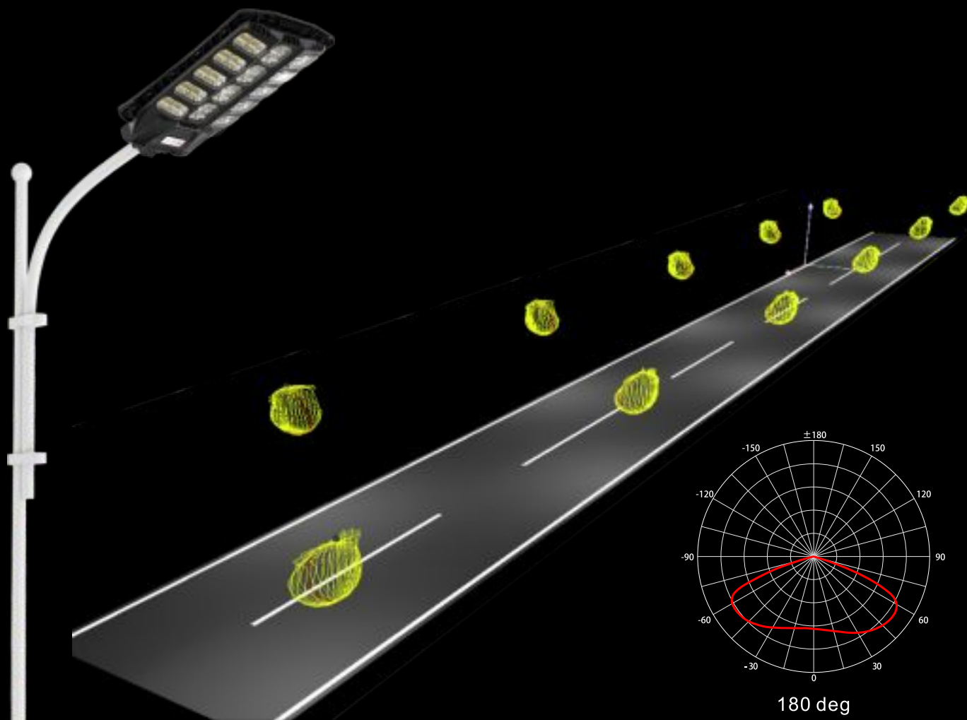
C Plane Lighting Distributions
